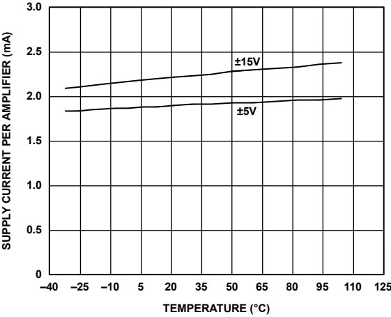
Figure 40. AD8513 Supply Current per Amplifier vs. Temperature
