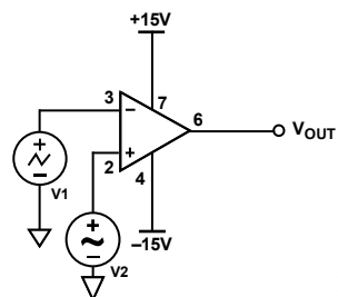
Figure 54. Pulse-Width Modulator
