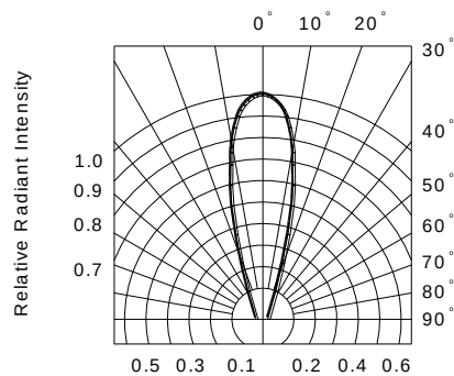
FIG.6 RADIATION DIAGRAM
