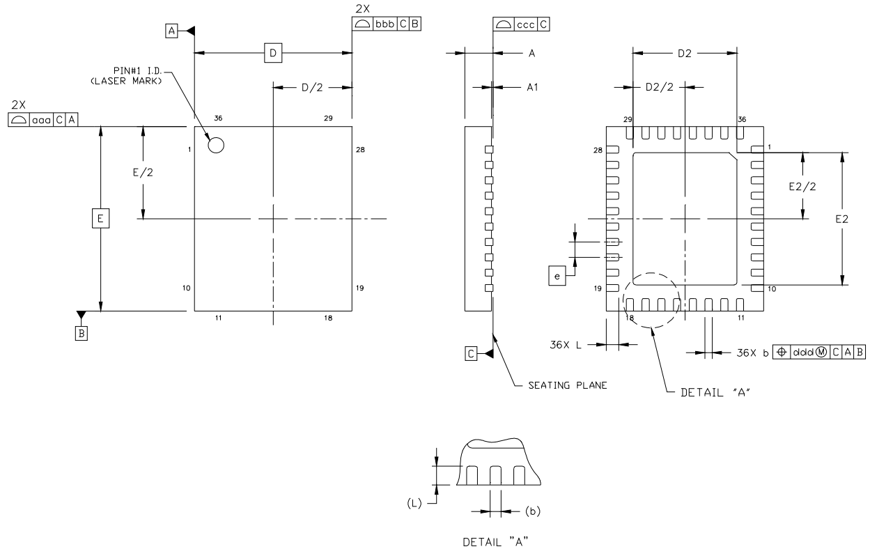
Figure 3.4. QFN-36 Package Drawing
