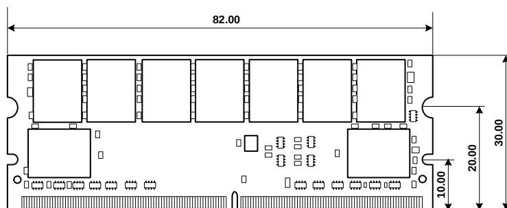
Figure: mechanical dimensions 1
