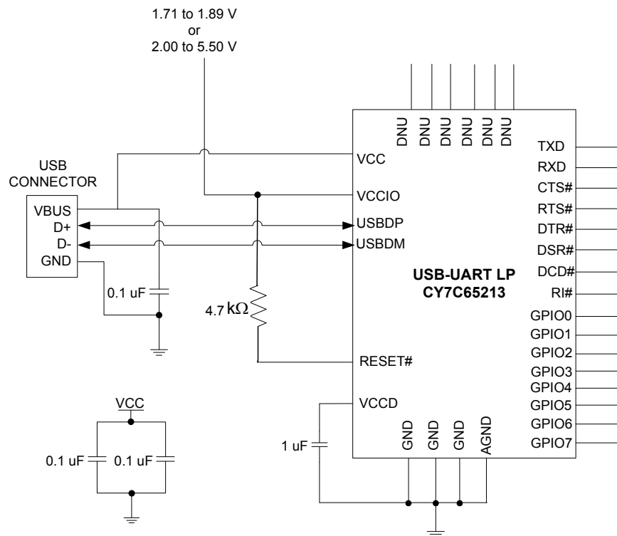
Figure 2. Self-Powered Configuration
