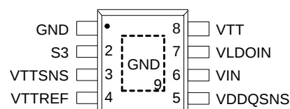
SOP-8 (Exposed Pad)
