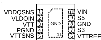
WDFN-10L 3x3
