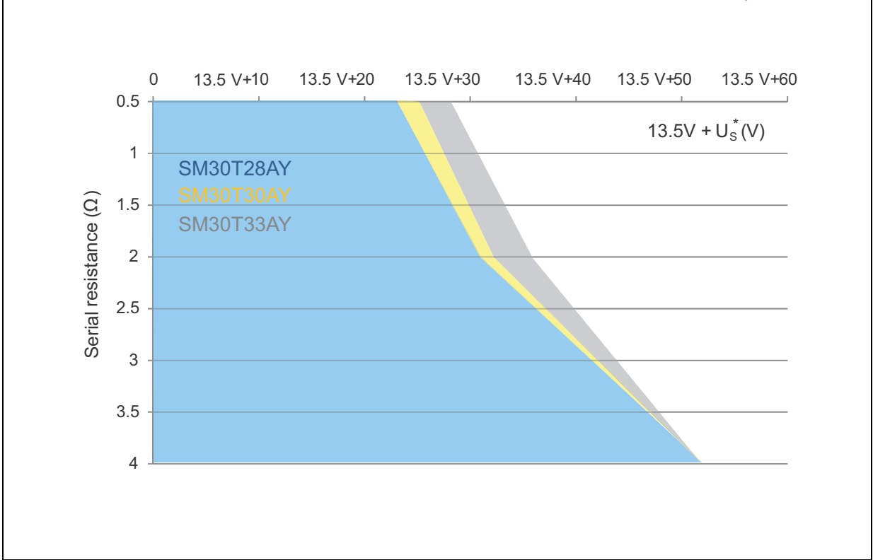
Figure 17. Load dump capability (typical values, U_s^* = f(R_i) pulse 5b, U_s = 87\text{ V} , t_p = 150\text{ ms} )
