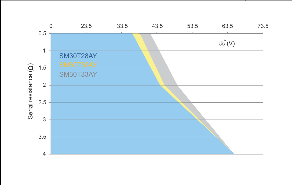
Figure 20. Load dump capability (typical values, U_s^* = f(R_i) test B, U_s = 87\text{ V} , t_p = 150\text{ ms} )
