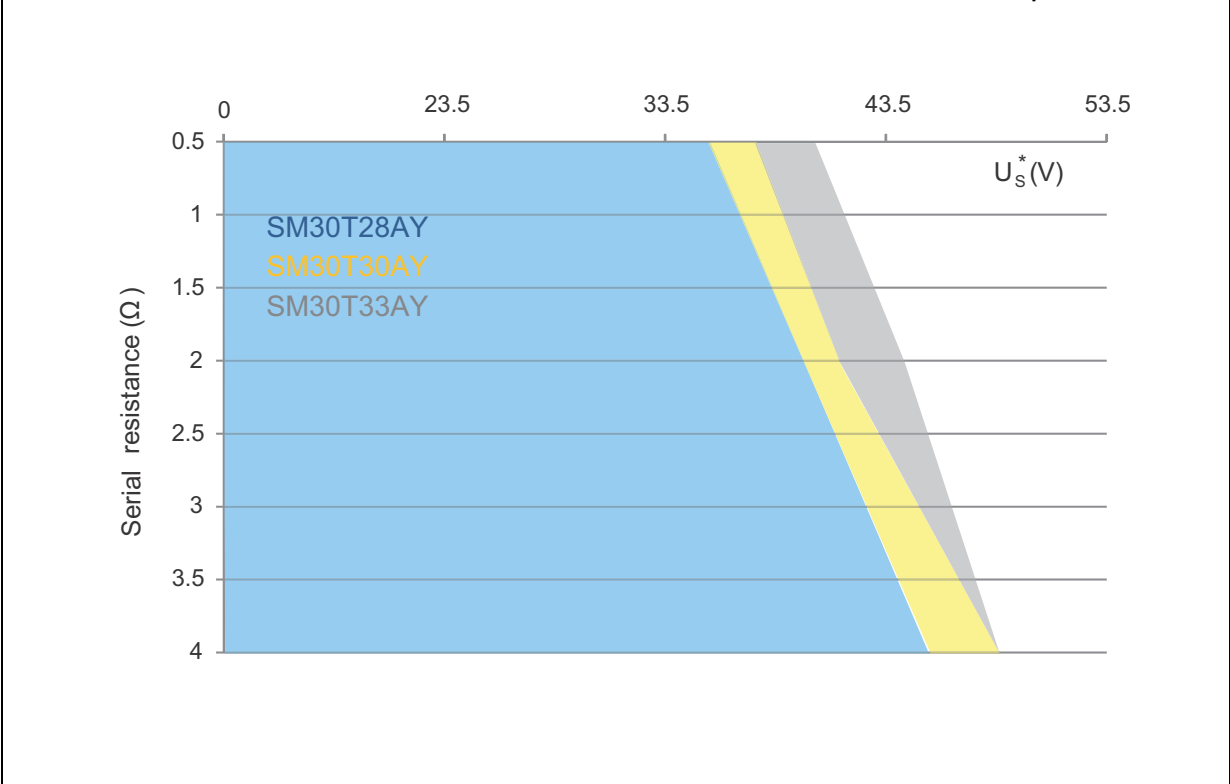
Figure 21. Load dump capability (typical values, U_s^* = f(R_i) test B, U_s = 87\text{ V} , t_p = 400\text{ ms} )
