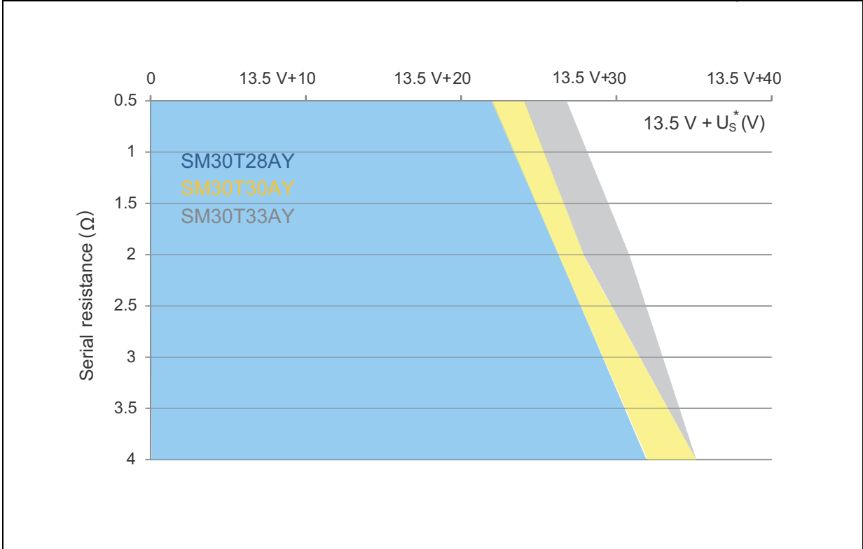
Figure 18. Load dump capability (typical values, U_s^* = f(R_i) pulse 5b, U_s = 87\text{ V} , t_p = 400\text{ ms} )
