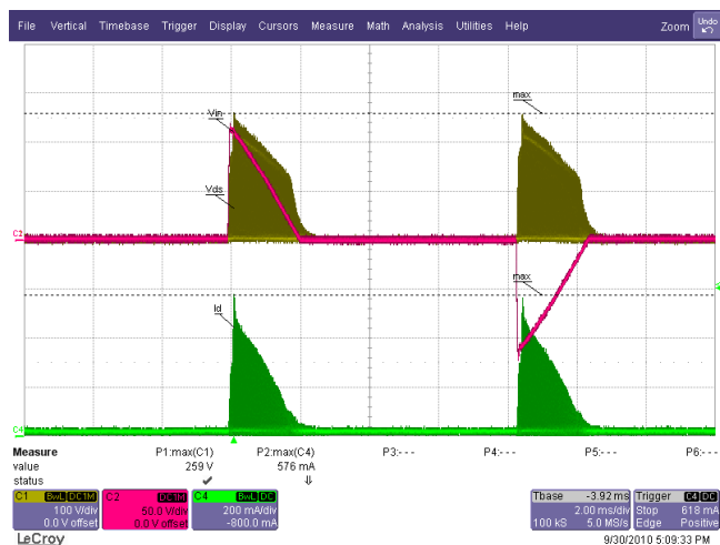
Figure 39 – 115 VAC / 60 Hz, 135° Dimming Phase Angle. 6 LED in Series (18.2 V / 350 mA) Ch1(Yellow): V_{DS} , 100 V / div. Ch2(Red): V_{IN} , 50 V / div. Ch4(Green): I_{DS} , 200 mA / div., 2 ms / div.
