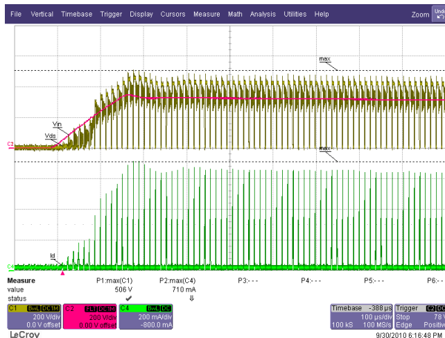
Figure 44 – 230 VAC / 50 Hz, 90° Dimming Phase Angle. 6 LED in Series (18.2 V / 350 mA) Ch1(Yellow): V_{DS} , 200 V / div. Ch2(Red): V_{IN} , 200 V / div. Ch4(Green): I_{DS} , 200 mA / div., 100 μs / div.
