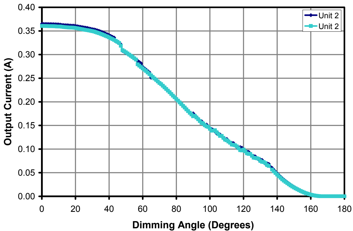
Figure 20 – Sample Curve for Unit to Unit Output Current Dimming Performance at 230 V / 50 Hz.
