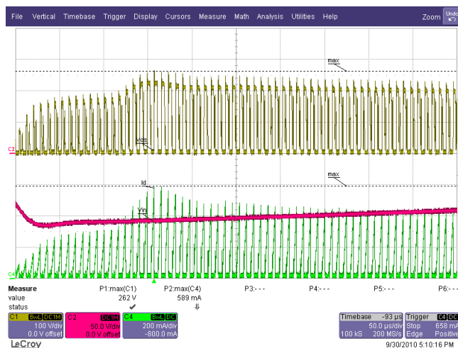
Figure 40 – 115 VAC / 60 Hz, 135° Dimming Phase Angle. 6 LED in Series (18.2 V / 350 mA) Ch1(Yellow): V_{DS} , 100 V / div. Ch2(Red): V_{IN} , 50 V / div. Ch4(Green): I_{DS} , 200 mA / div., 50 \mu s / div.
