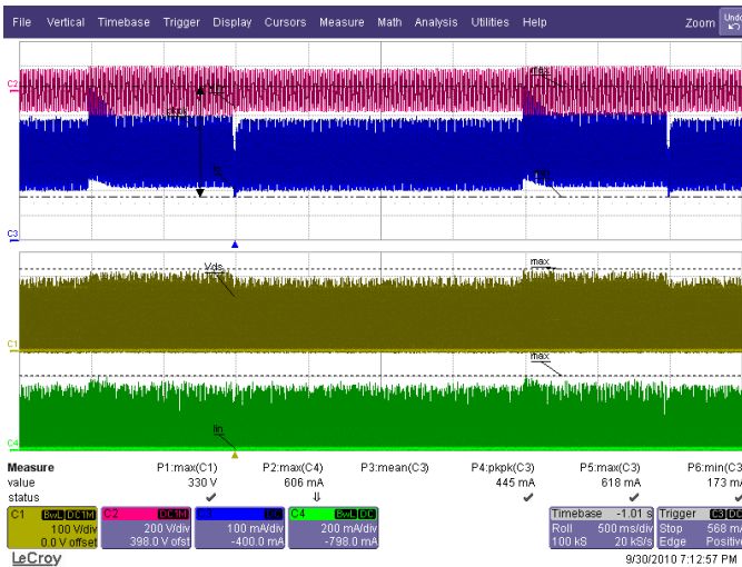
Figure 69 – 115-132-115 VAC / 60 Hz. 5 LED in Series (15 V). Ch1(Yellow): V_{DS} , 100 V / div. Ch2(Red): V_{IN} , 200 V / div. Ch3(Blue): I_O , 100 mA / div. Ch4(Green): I_{DS} , 200 mA / div., 500 ms / div.
