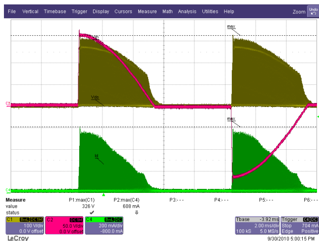
Figure 37 – 115 VAC / 60 Hz, 90° Dimming Phase Angle. 6 LED in Series (18.2 V / 350 mA) Ch1(Yellow): V_{DS} , 100 V / div. Ch2(Red): V_{IN} , 50 V / div. Ch4(Green): I_{DS} , 200 mA / div., 2 ms / div.
