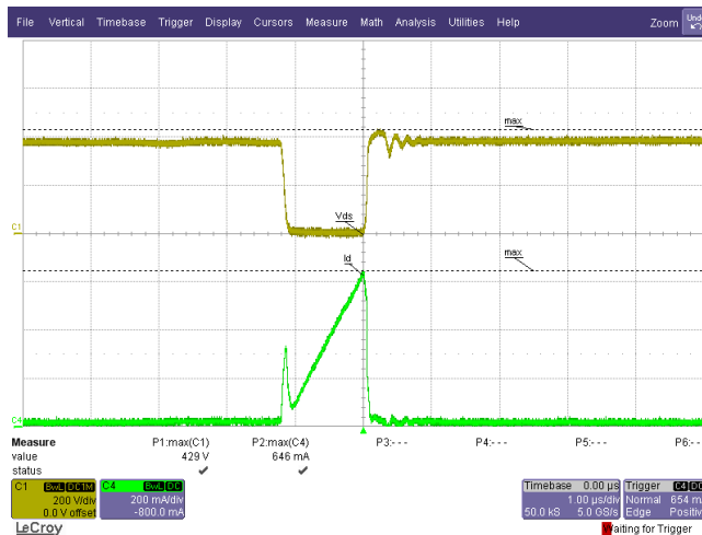
Figure 48 – 265 VAC. Load Shorted. Upper: V_{DRAIN} , 200 V / div. Lower: I_{DRAIN} , 0.2 A / div., 1 \mu s / div.
