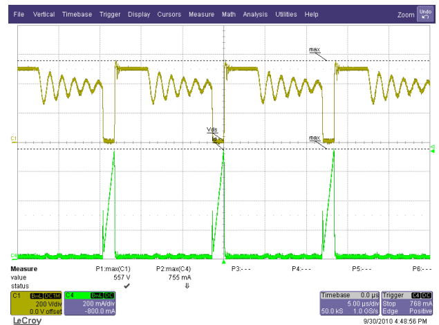
Figure 32 – 265 VAC / 63 Hz, 6 LED in Series (18.2 V / 350 mA). Upper: V_{DRAIN} , 200 V / div., 5 μs / div. Lower: I_{DRAIN} , 0.2 A / div.
