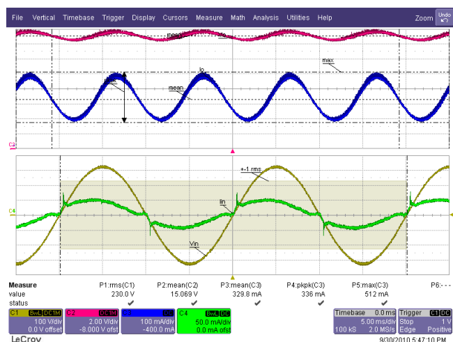
Figure 57 – 230 VAC / 50 Hz. 5 LED in Series (15 V). Ch1(Yellow): V_{IN} , 100 V / div. Ch2(Red): V_O , 2 V / div. Ch3(Blue): I_O , 100 mA / div. Ch4(Green): I_{IN} , 50 mA / div., 5 ms / div.
