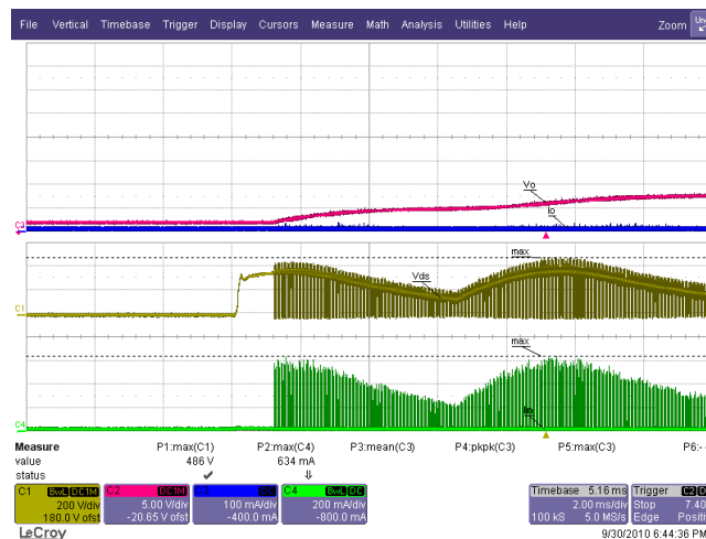
Figure 34 – 265 VAC / 63 Hz, 6 LED in Series (18.2 V / 350 mA). Ch1(Yellow): V_{DS} , 200 V / div. Ch2(Red): V_O , 5 V / div. Ch3(Blue): I_O , 100 mA / div. Ch4(Green): I_{DS} , 200 mA / div., 2 ms / div.
