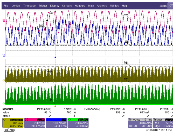
Figure 78 – 230-265-230 VAC / 50 Hz. 5 LED in Series (15 V). Ch1(Yellow): V_{DS} , 200 V / div. Ch2(Red): V_{IN} , 200 V / div. Ch3(Blue): I_O , 100 mA / div. Ch4(Green): I_{DS} , 200 mA / div., 50 ms / div.
