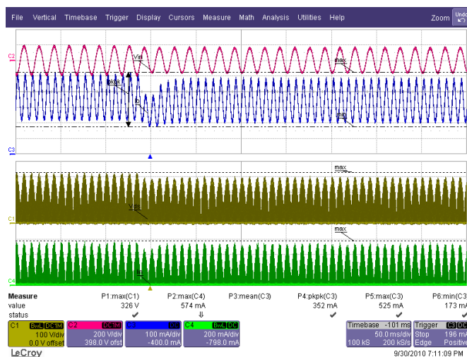
Figure 72 – 115-132-115 VAC / 60 Hz. 5 LED in Series (15 V). Ch1(Yellow): V_{DS} , 100 V / div. Ch2(Red): V_{IN} , 200 V / div. Ch3(Blue): I_O , 100 mA / div. Ch4(Green): I_{DS} , 200 mA / div., 50 ms / div.
