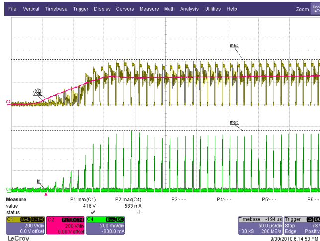
Figure 42 – 230 VAC / 50 Hz, 45° Dimming Phase Angle. 6 LED in Series (18.2 V / 350 mA) Ch1(Yellow): V_{DS} , 200 V / div. Ch2(Red): V_{IN} , 200 V / div. Ch4(Green): I_{DS} , 200 mA / div., 50 μs / div.
