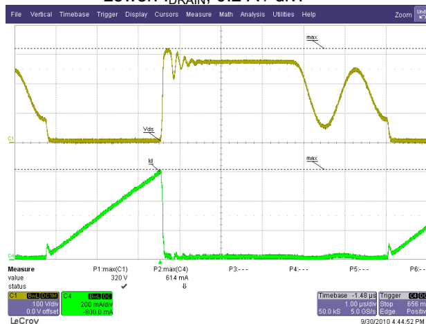
Figure 28 – 115 VAC / 60 Hz, 6 LED in Series (18.2 V / 350 mA). Upper: V_{DRAIN} , 100 V / div., 1 μs / div. Lower: I_{DRAIN} , 0.2 A / div.
