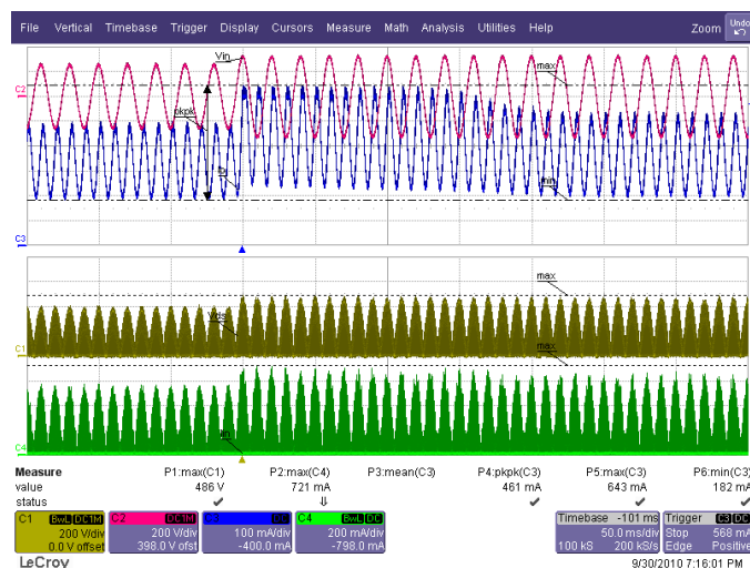
Figure 75 – 230-180-230 VAC / 50 Hz. 5 LED in Series (15 V). Ch1(Yellow): V_{DS} , 200 V / div. Ch2(Red): V_{IN} , 200 V / div. Ch3(Blue): I_O , 100 mA / div. Ch4(Green): I_{DS} , 200 mA / div., 50 ms / div.
