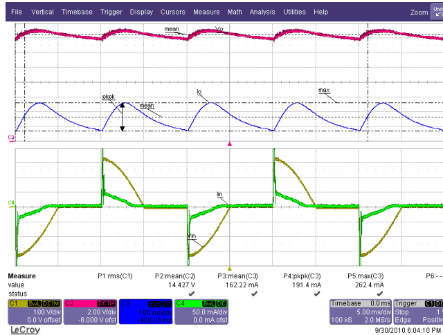
Figure 62 – 230 VAC / 50 Hz.
