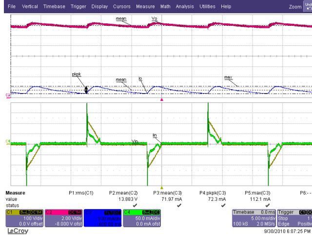
Figure 64 – 230 VAC / 50 Hz.
