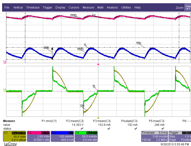
Figure 61 – 115 VAC / 60 Hz.
