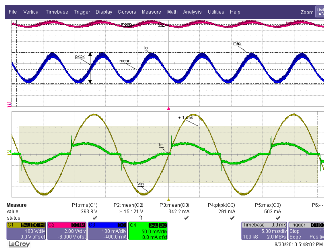
Figure 58 – 265 VAC / 63 Hz. 5 LED in Series (15 V). Ch1(Yellow): V_{IN} , 100 V / div. Ch2(Red): V_O , 2 V / div. Ch3(Blue): I_O , 100 mA / div. Ch4(Green): I_{IN} , 50 mA / div., 5 ms / div.
