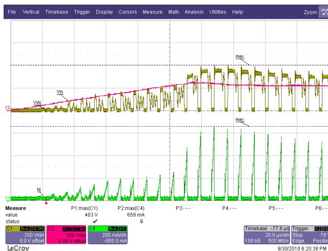
Figure 46 – 230 VAC / 50 Hz, 135° Dimming Phase Angle. 6 LED in Series (18.2 V / 350 mA) Ch1(Yellow): V_{DS} , 200 V / div. Ch2(Red): V_{IN} , 200 V / div. Ch4(Green): I_{DS} , 200 mA / div., 20 \mu s / div.
