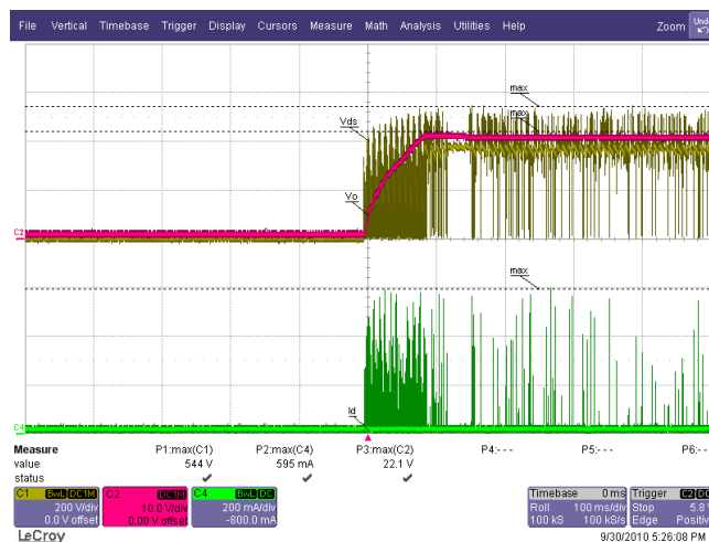
Figure 50 – 265 VAC. Load Open. Ch1(Yellow): V_{DS} , 200 V / div. Ch2(Red): V_O , 10 V / div. Ch4(Green): I_{DS} , 200 mA / div., 20 μs / div.
