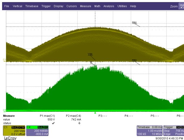
Figure 31 – 265 VAC / 63 Hz, 6 LED in Series (18.2 V / 350 mA). Upper: V_{DRAIN} , 200 V / div., 1 ms / div. Lower: I_{DRAIN} , 0.2 A / div.
