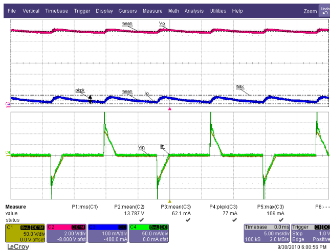
Figure 63 – 115 VAC / 60 Hz.
