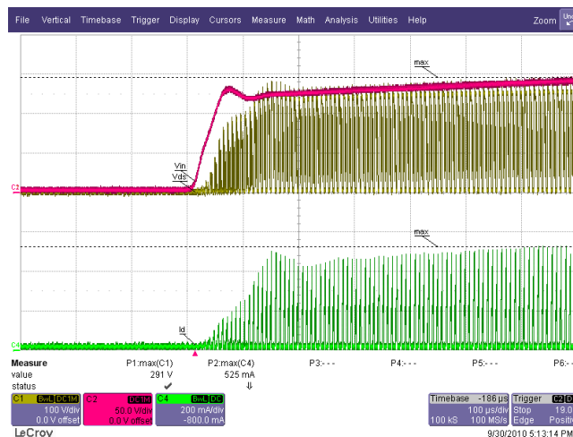
Figure 36 – 115 VAC / 60 Hz, 45° Dimming Phase Angle. 6 LED in Series (18.2 V / 350 mA). Ch1(Yellow): V_{DS} , 100 V / div. Ch2(Red): V_{IN} , 50 V / div. Ch4(Green): I_{DS} , 200 mA / div., 100 \mu s / div.
