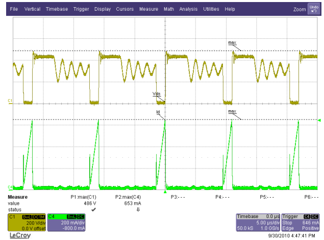
Figure 30 – 230 VAC / 50 Hz, 6 LED in Series (18.2 V / 350 mA). Upper: V_{DRAIN} , 200 V / div., 5 μs / div. Lower: I_{DRAIN} , 0.2 A / div.
