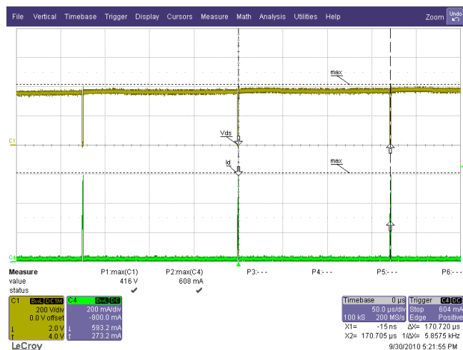
Figure 49 – 265 VAC. Load Shorted. Upper: V_{DRAIN} , 200 V / div. Lower: I_{DRAIN} , 0.2 A / div., 50 μs / div.
