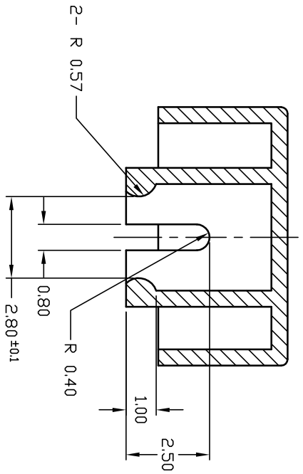
SECTION Y-Y DETAIL
