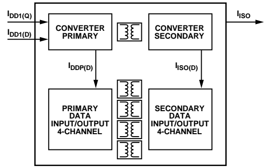
Figure 31. Power Consumption Within the ADuM640x
