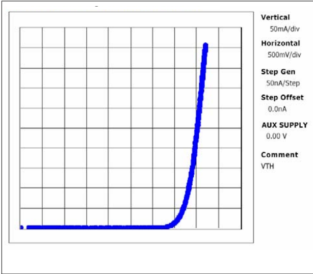
Figure 5. Threshold voltage
