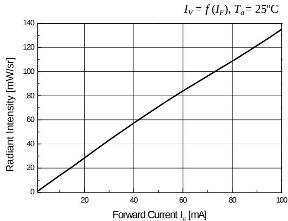
Forward Current vs. Radiant Intensity
