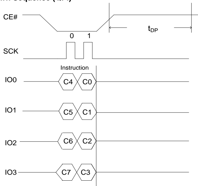
Figure 8.35 Deep Power Down Sequence (QPI)
