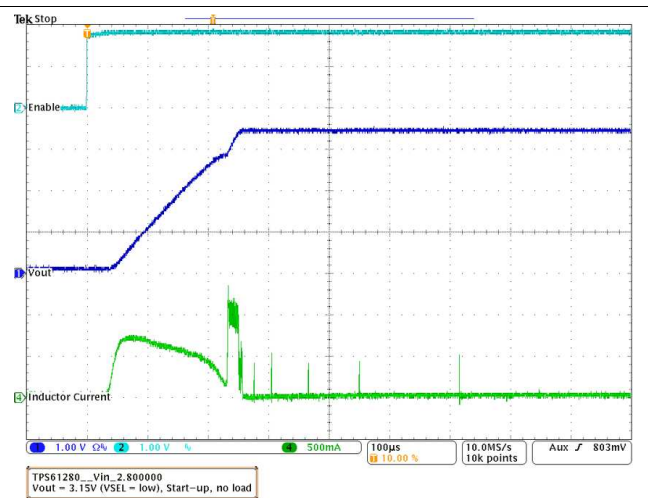
Figure 46. Start-Up at No Load
