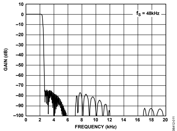
Figure 11. DAC Stop-Band Filter Response
