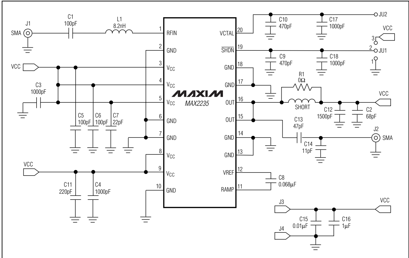
Figure 1. MAX2235 EV Kit Schematic
