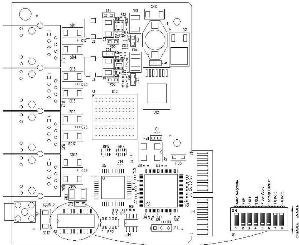
iMcV-LIM with SFP and Configuration Control
