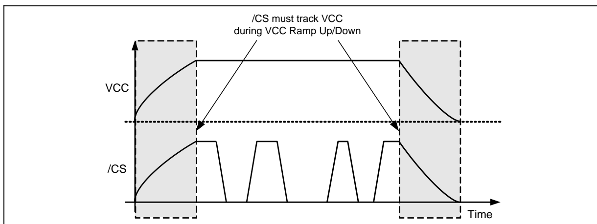
Figure 37b. Power-up, Power-Down Requirement
