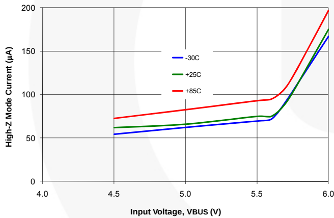
Figure 19. V_{\text{BUS}} Current in High-Impedance Mode with Battery Open
