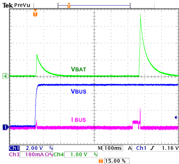
Figure 17. No Battery at V_{\text{BUS}} Power-up; FAN5400, FAN5403 Figure 18. No Battery at V_{\text{BUS}} Power-up; FAN5402, FAN5405
