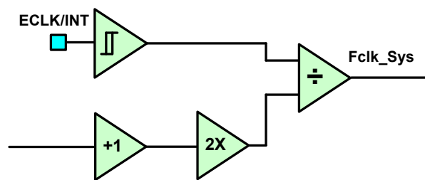
FIGURE 37. SIMPLIFIED INTERNAL BLOCK CONNECTION OF THE ECLK/INT PIN
