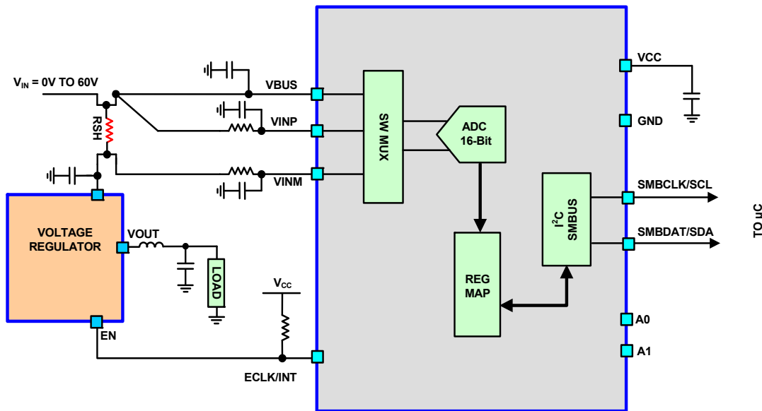
FIGURE 1. TYPICAL APPLICATION
