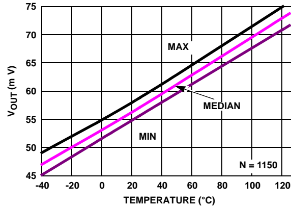
FIGURE 37. V_{OUT} LOW vs TEMPERATURE, V_+ = 5V , V_- = 0V , V_{CM} = 2.5V , R_L = \text{Open} (Continued)
