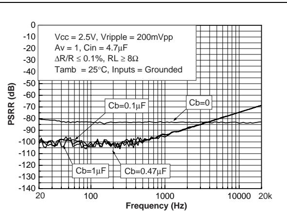
Figure 74. PSRR vs. frequency with random choice condition
