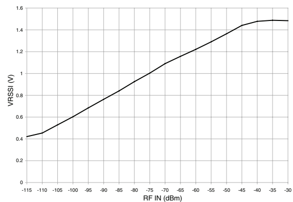
Figure 7: RSSI Curve
