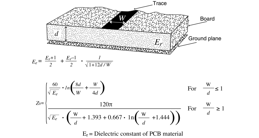
Figure 27: Microstrip Formulas
