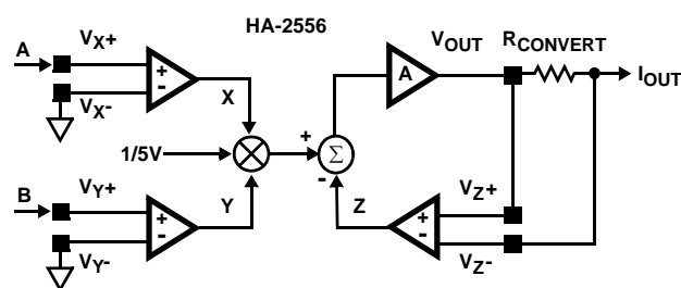
FIGURE 10. CURRENT OUTPUT
