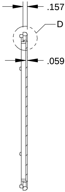
SECTION C-C
