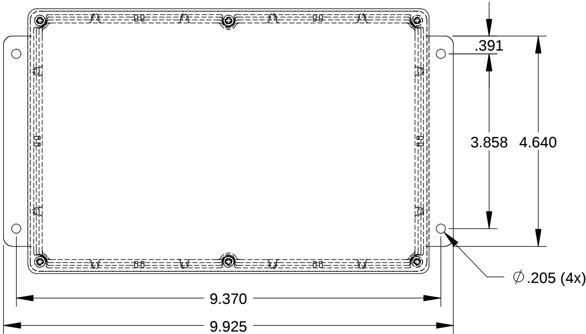
SECTION B-B
