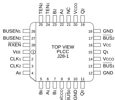
28-Pin PLCC (J28-1)
