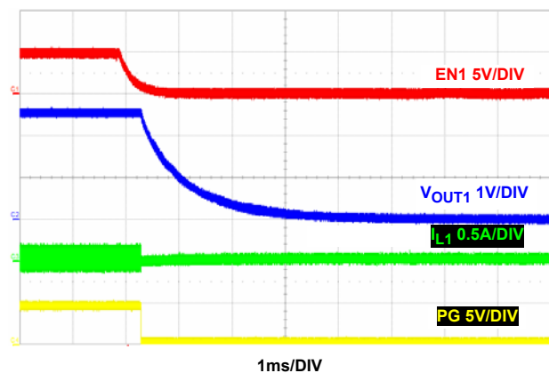
FIGURE 30. SOFT-DISCHARGE SHUTDOWN CHANNEL 1
