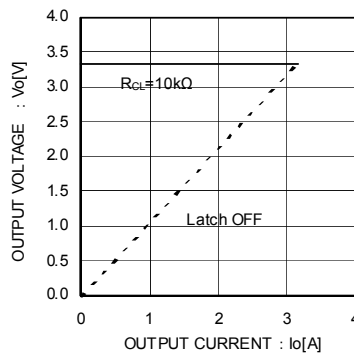
Fig.8 Load regulation
