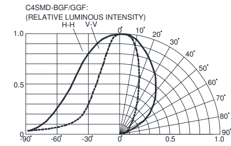
FIG.6a BLUE&GREEN FAR FIELD PATTERN
