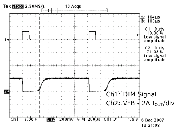
Fig. 14: 1.1KHz, 10% Duty Cycle Dimming Signal Dimming Signal is ~70% LED Duty Cycle
