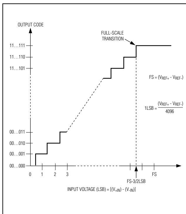
Figure 10. Ideal Input Voltages and Output Codes
