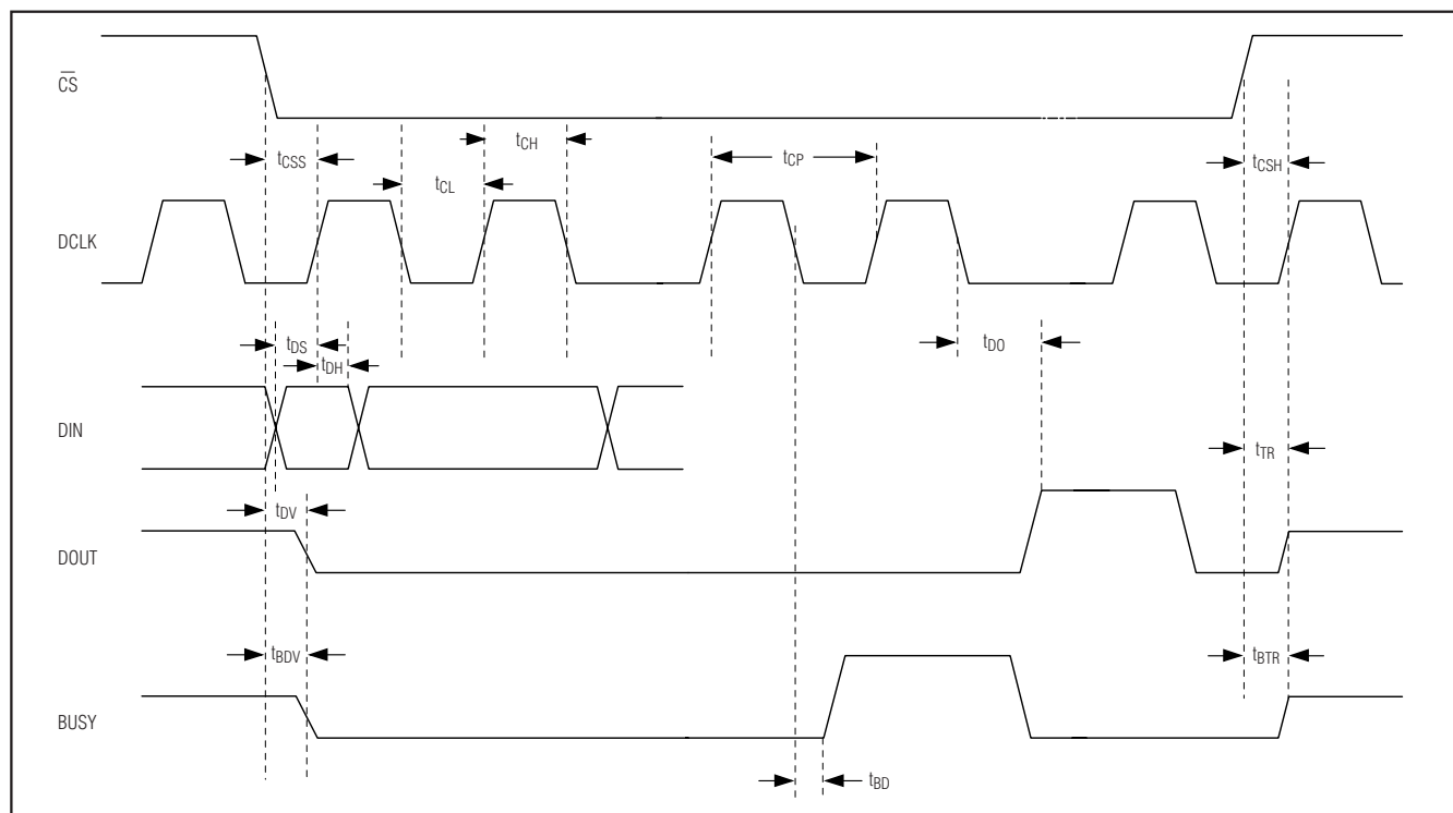
Figure 1. Detailed Serial Interface Timing
