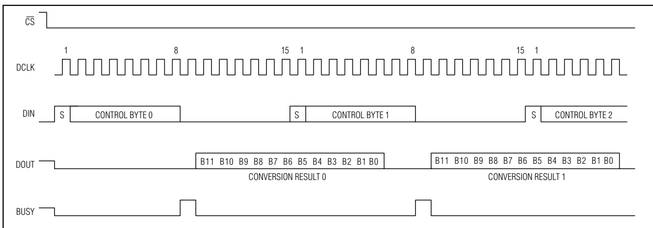
Figure 8. 15-Clock/Conversion Timing
