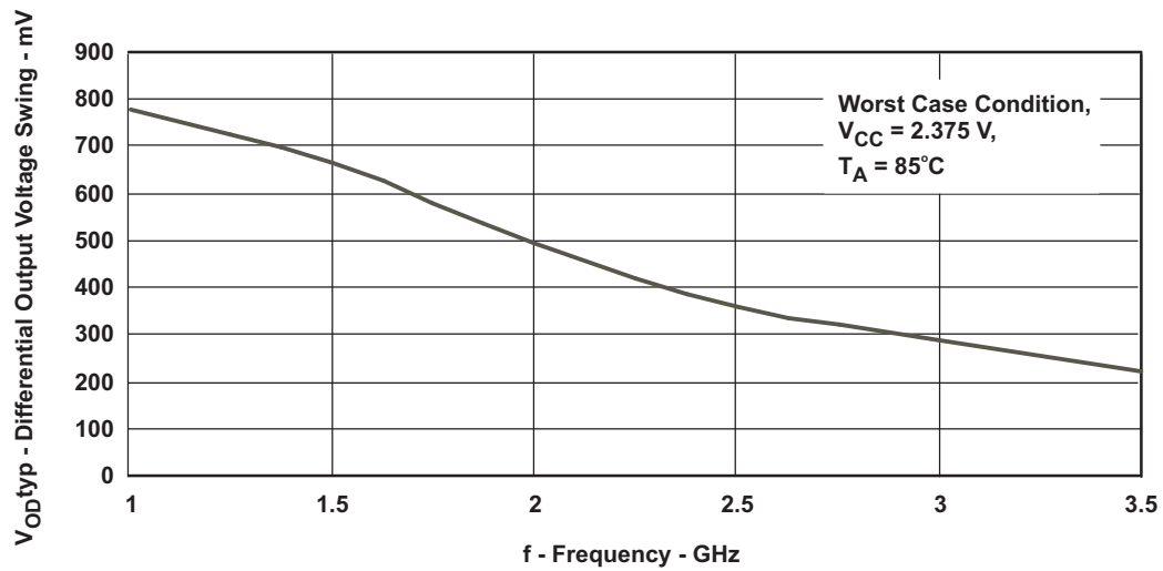
Figure 4. LVPECL Input Using CLK0 Pair, V_{CM} = 1\text{ V} , V_{ID} = 0.5\text{ V}
