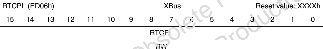
Figure 73. Prescaler registers
