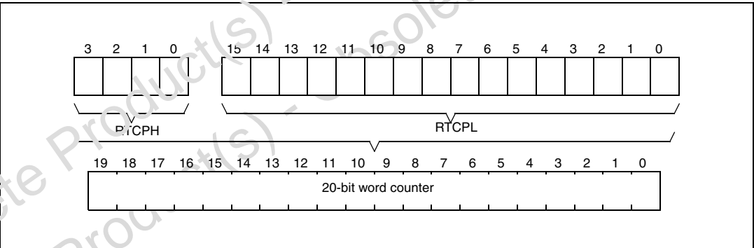
Figure 73. Prescaler registers
