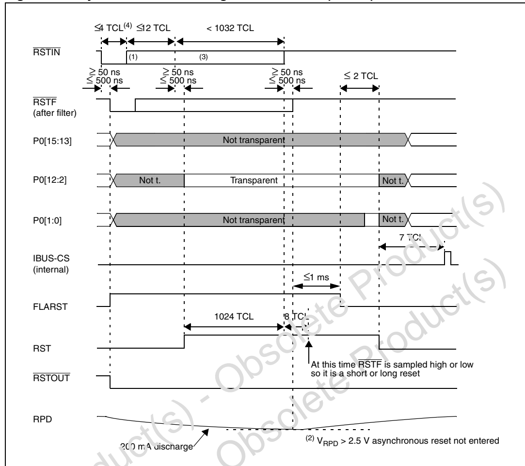
Figure 79. Synchronous short/long hardware reset ( \overline{\text{EA}} = 1 )
