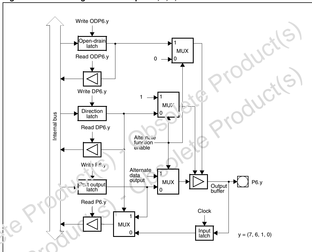
Figure 50. Block diagram of Port 6 pins 7, 6, 1, 0
