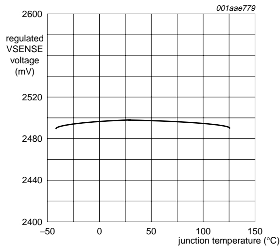
Fig 4. Typical regulated V SENSE voltage versus junction temperature
