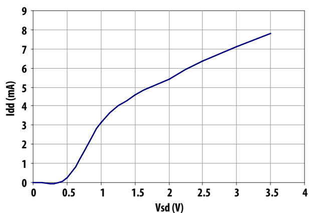
Figure 6. Idd vs Vsd for Vdd = 2.8V, R2 = 3.9k Ohm
