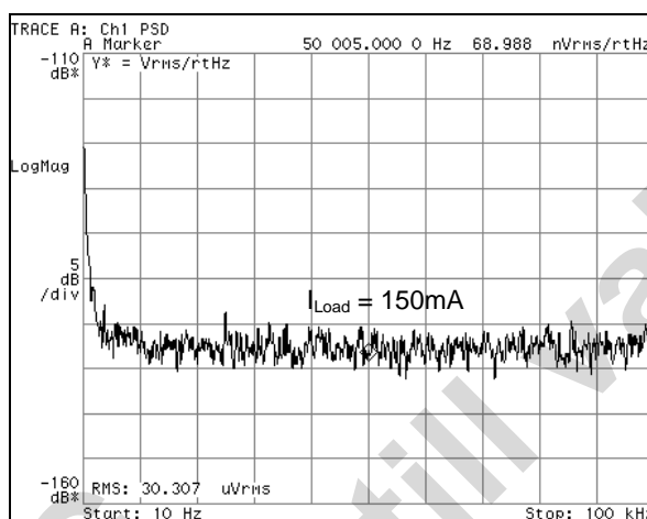
Figure 16. Output Noise of LDOs VANA_1, VANA_2, VRF_1, VRF_2
