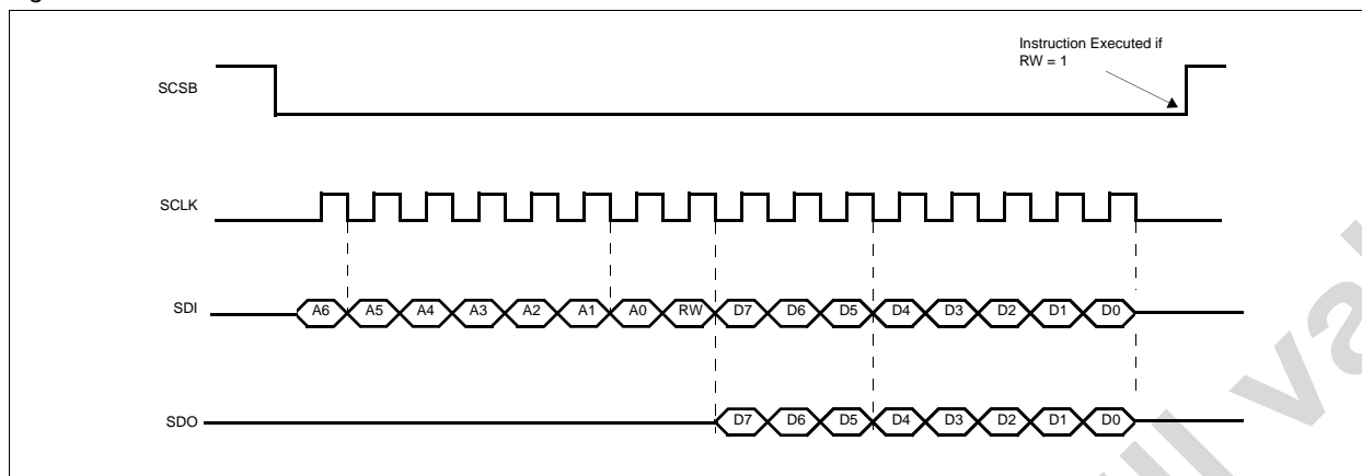
Figure 28. SPI Waveform
