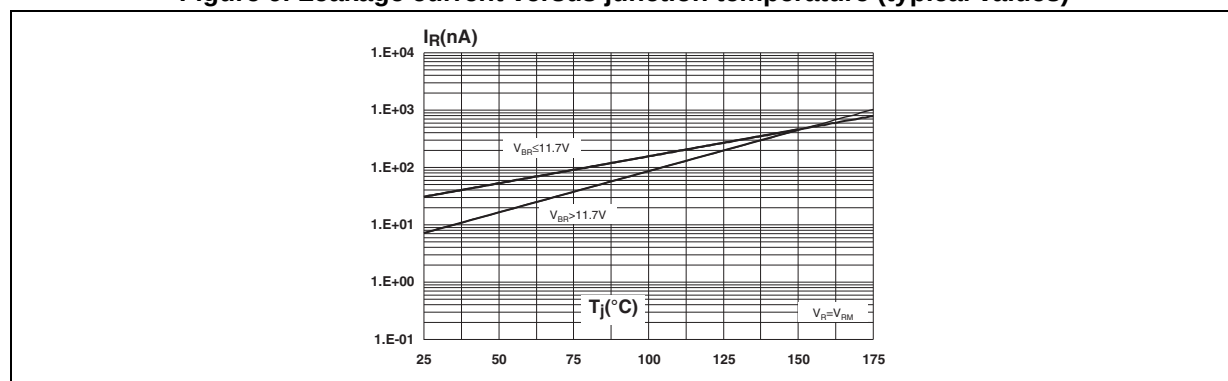
Figure 9. Leakage current versus junction temperature (typical values)
