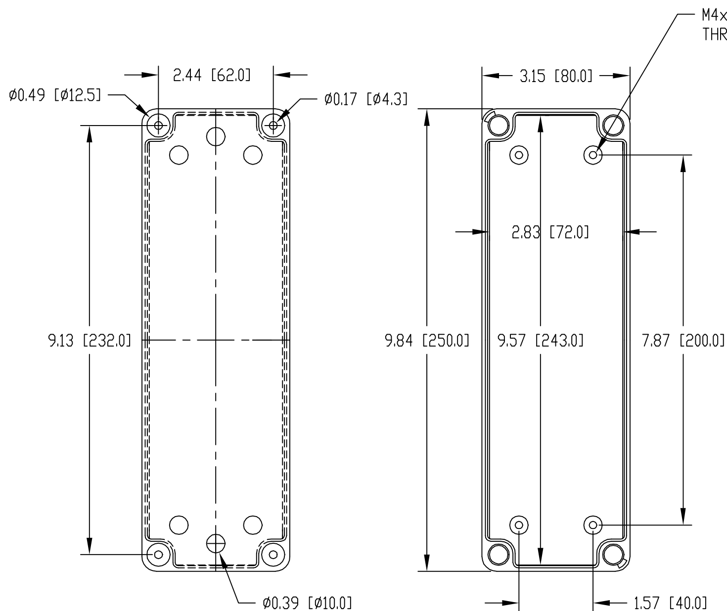
BOTTOM VIEW
