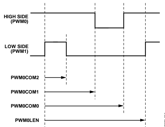
Figure 26. PWM Timing
