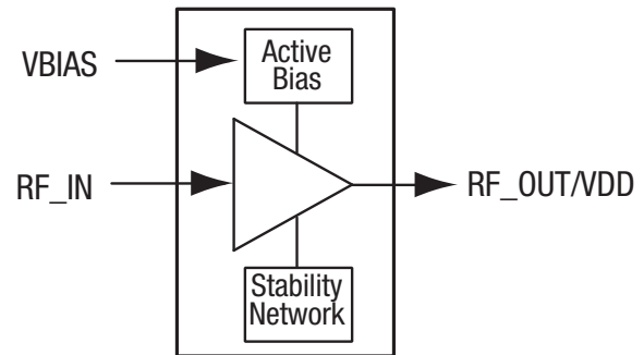
Figure 1. SKY67012-396LF Block Diagram
