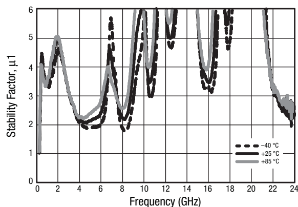
Figure 12. Stability Factor ( \mu_1 ) vs Frequency and Temperature, Wide Band
