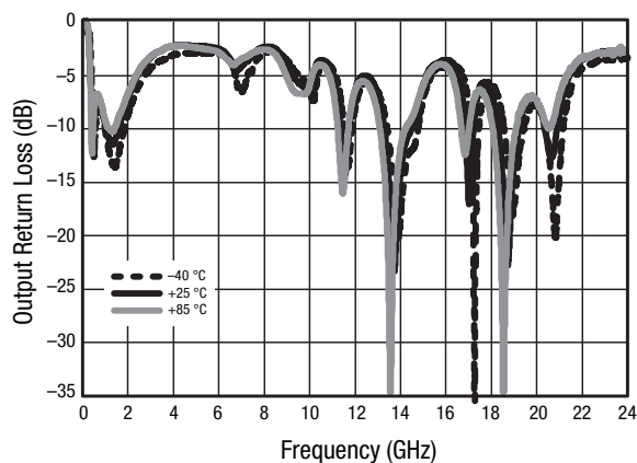
Figure 11. Small Signal Output Return Loss (IS22I) vs Frequency and Temperature, Wide Band
