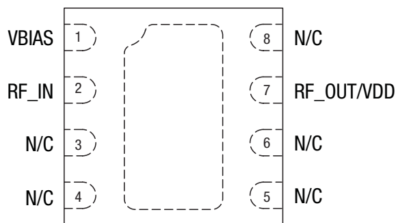
Figure 2. SKY67012-396LF Pinout – 8-Pin DFN (Top View)
