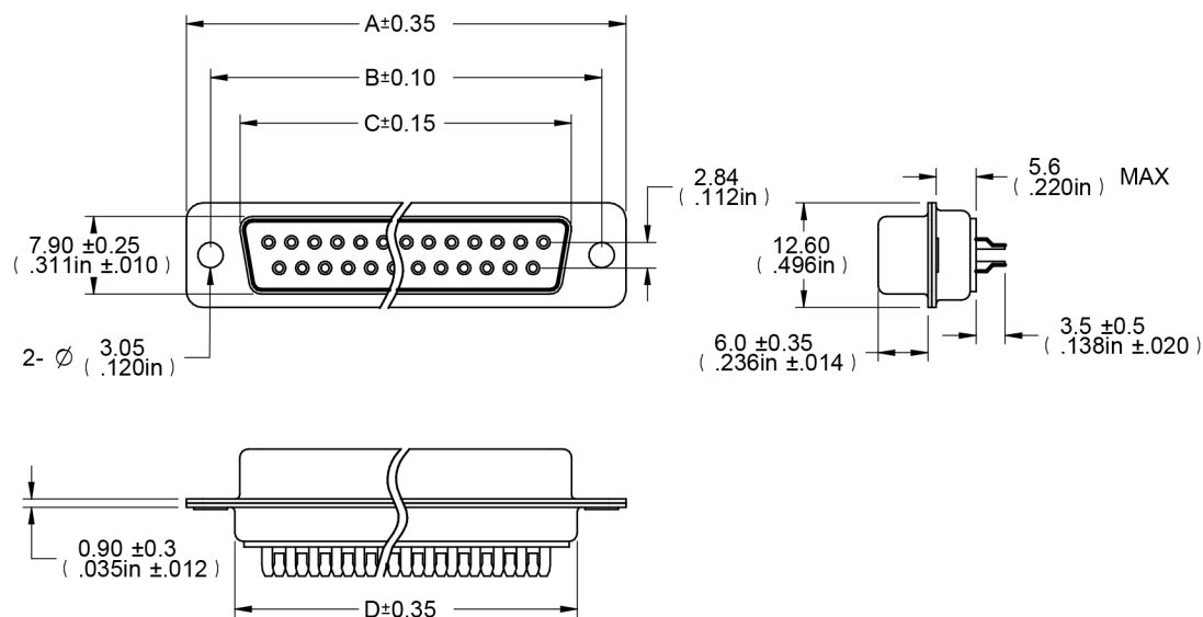
DIM OUTLINE
