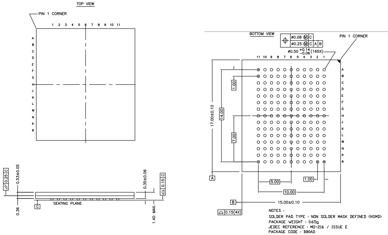
Figure 7. 165-ball FBGA (15 × 17 × 1.40 mm) (0.50 Ball Diameter) Package Outline, 51-85195
