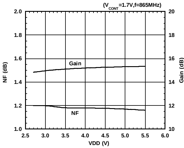
NF, Gain vs. VDD
