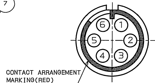
DETAIL B (SCALE 5:1) CONTACT ARRANGEMENT
