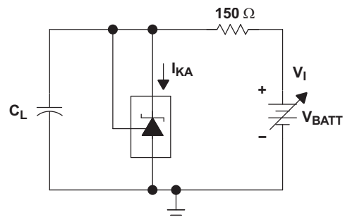
TEST CIRCUIT FOR CURVE A
