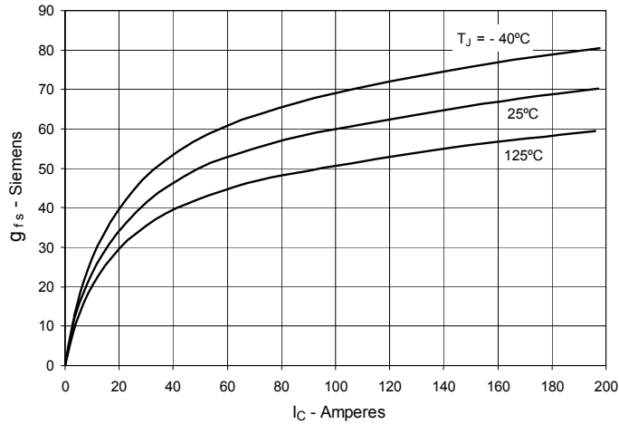
Fig. 7. Transconductance
