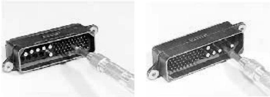
Extracting #20 & #16 Contacts
