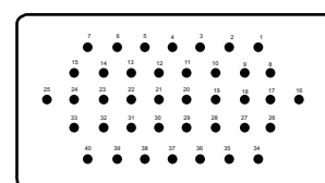
MOLDED 40 TOTAL CONTACTS:40 40-#16(#1-40) CLEARANCE 1/16 (1.59)
