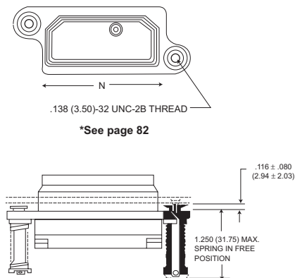
Mounting Style H - MIL-C-83733/12(USAF) Staggered Spring Mounting
