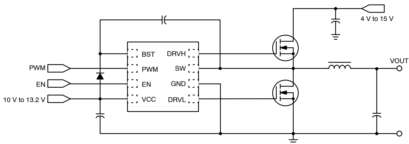
Figure 2. Typical Application
