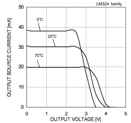
Fig. 30 Output Source Current - Output Voltage (VCC=5[V])
