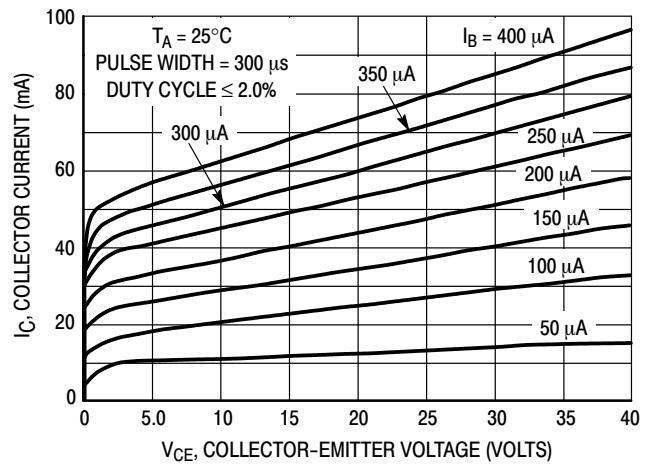
Figure 7. Collector Characteristics
